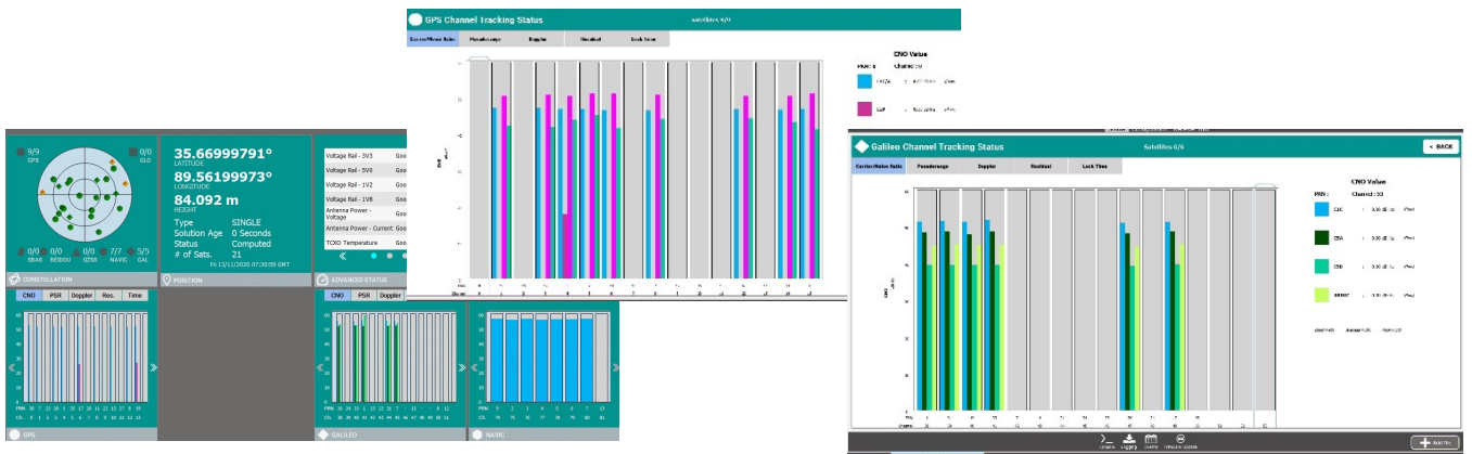
Novatel OEM7 working with the Replicator A1-R4-Q8-U3 dual/triple frequency GPS, Galileo, NavIC and GLONASS simulated signals.
